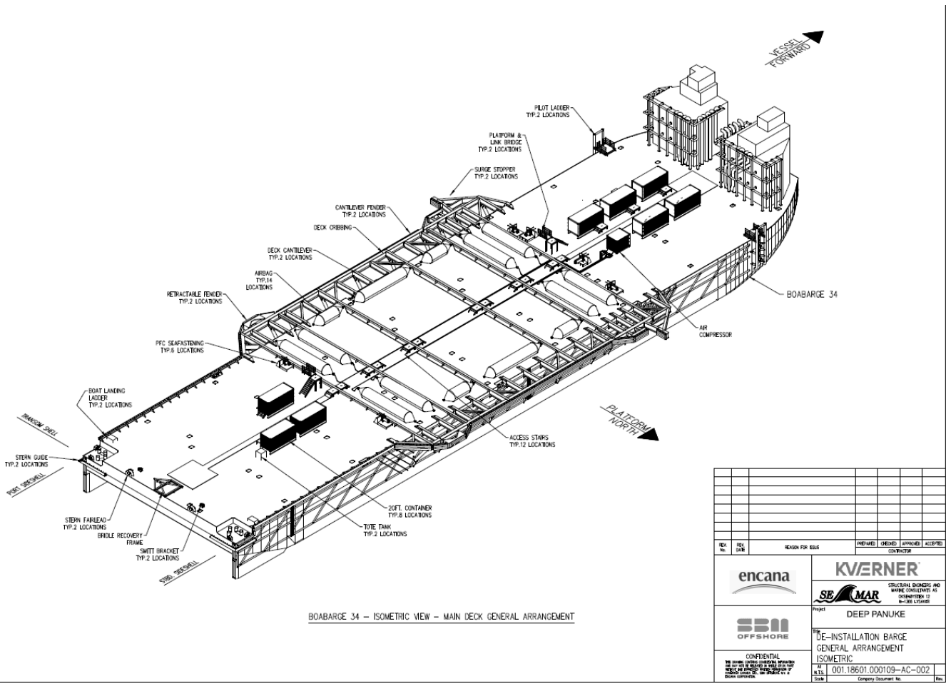
Figure 1. Isometric G.A.
